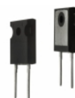
DSI45-12A IXYS DIODE GEN PURP 1.2KV 45A TO247AD
