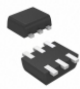
BCM857BV-7 Diodes Incorporated TRANS 2PNP 45V 0.1A SOT563
