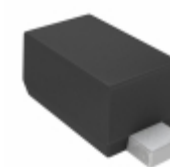
CDZVT2R8.2B Rohm Semiconductor DIODE ZENER 8.2V 100MW VMN2M
