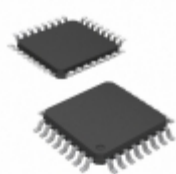
CY7C4241V-25AXCT Cypress Semiconductor Corp IC SYNC FIFO MEM 4KX9 32-TQFP
