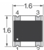
EHF-FD1541 Panasonic Electronic Components DIRECTIONAL COUPLER 1850MHZ-14DB
