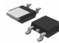
LP2950CDT-3.3 ON Semiconductor IC REG LDO 3.3V 0.1A DPAK
