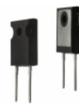
DSEP60-025A IXYS DIODE GEN PURP 250V 60A TO247AD
