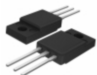
BTA202X-600E,127 WeEn Semiconductors TRIAC SENS GATE 600V 2A TO220-3
