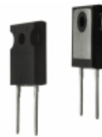
DSEP60-06A IXYS DIODE GEN PURP 600V 60A TO247AD
