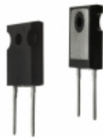
DSEP60-12A IXYS DIODE GEN PURP 1.2KV 60A TO247AD
