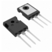
DPG60C200HB IXYS DIODE ARRAY GP 200V 30A TO247AD
