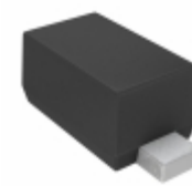
CDZVT2R3.6B Rohm Semiconductor DIODE ZENER 3.6V 100MW VMN2M
