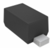
CDZVT2R2.2B Rohm Semiconductor DIODE ZENER 2.2V 100MW VMN2M
