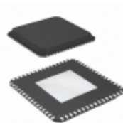
DSPIC33EP64MC506T-I/MR Micrel / Microchip Technology IC MCU 16BIT 64KB FLASH 64QFN
