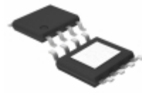
BDJ0GA5WEFJ-E2 LAPIS Semiconductor IC REG LDO 10V 0.5A 8HTSOP-J
