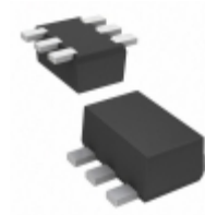
DMC964070R Panasonic TRANS PREBIAS DUAL NPN SSMINI6
