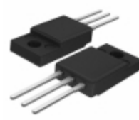
BTA312X-600E,127 WeEn Semiconductors TRIAC SENS GATE 600V 12A TO220-3
