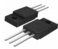
BTA312X-600C,127 WeEn Semiconductors TRIAC 600V 12A TO220F
