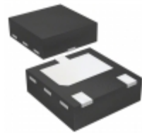
BC69-16PA,115 Nexperia USA Inc. TRANSISTOR PNP 20V 2A SOT1061
