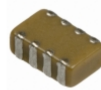
W2A43A180KAT2A AVX Corporation CAP ARRAY 18PF 25V NP0 0508
