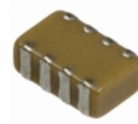
W2A43A330KAT2A AVX Corporation CAP ARRAY 33PF 25V NP0 0508
