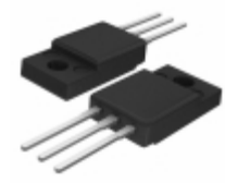
BTA312X-600B,127 WeEn Semiconductors TRIAC 600V 12A TO220F
