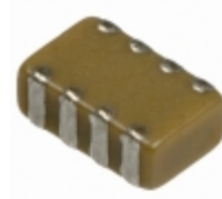
W2A45A100JAT2A AVX Corporation CAP ARRAY 10PF 50V NP0 0508
