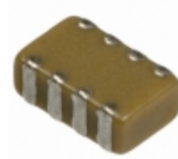
W2A43C221MAT2A AVX Corporation CAP ARRAY 220PF 25V X7R 0508
